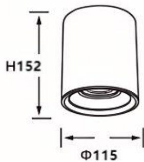
IP54 VERSION
